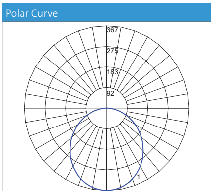
NORMALISED POLAR CURVE Maximum Candela = 366.607 cd/klm # 1. Vertical Plane Through Horizontal Angles (0 - 180)
